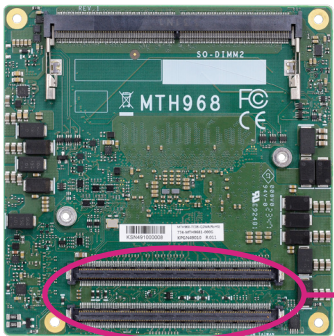
COM Express connector on MTH968
