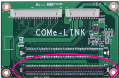
COM Express Connector
