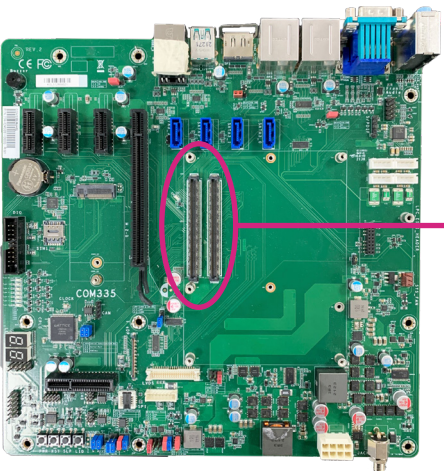
COM Express connector on the carrier board
