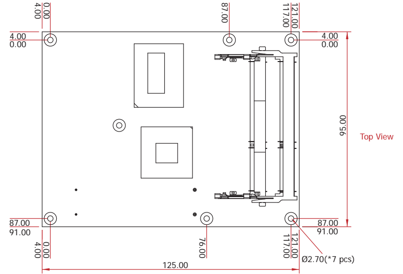
CR902-B/BL Series Module
