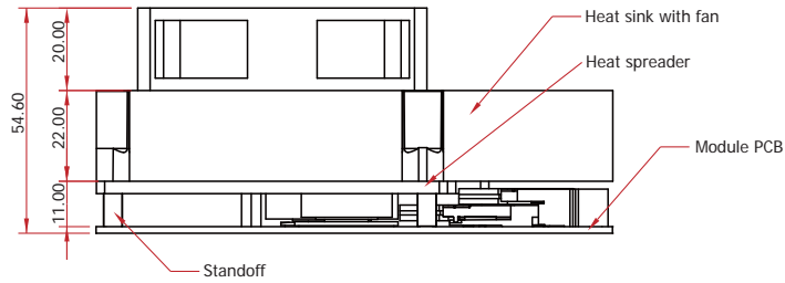
Side View of the Module with Heat Sink and Carrier Board
