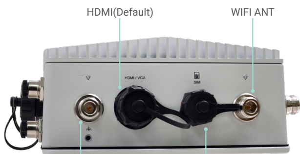
HDMI(Default) WIFI ANT WIFI ANT External SIM slot Right View
