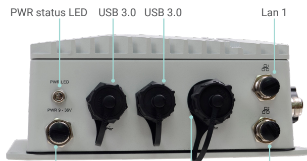
PWR status LED USB 3.0 USB 3.0 Lan 1 PWR 9~36V Combo (COM 1/2, CAN 1/2) Lan 2 Bottom View
