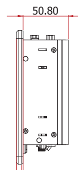
Right View
