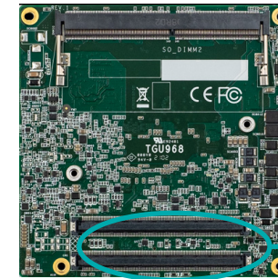
COM Express connector on TGU968
